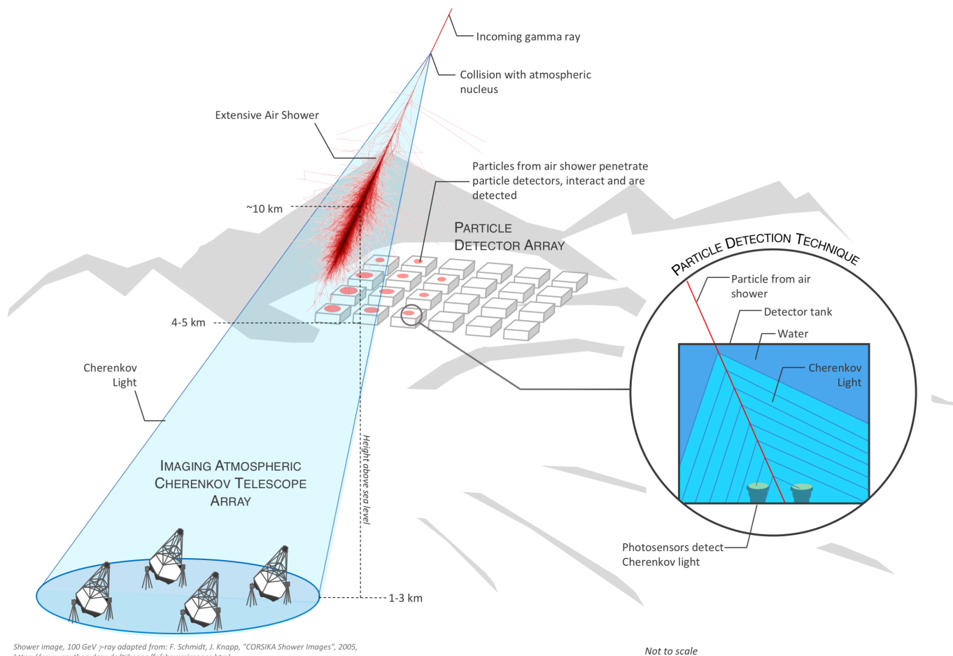
Illustration of the complementary detection techniques of high-energy gamma rays on ground.
